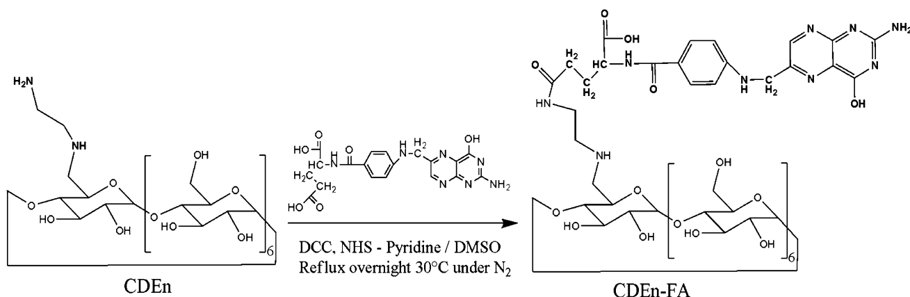
Scheme 1 Synthesis of CDEn-FA conjugate obtained by reaction between CDEn and FA (only the \alpha -isomer is reported)
