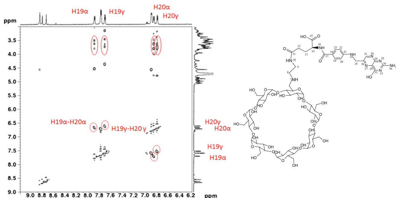
Fig. 1 Left: ROESY spectrum of CDEn-FA in D 2 O, T = 298 K. The cross peaks between H-19 \alpha and H-20 \alpha as well between H-19 \gamma and H-20 \gamma are evidenced (H-23 and H-22 are omitted because they are
